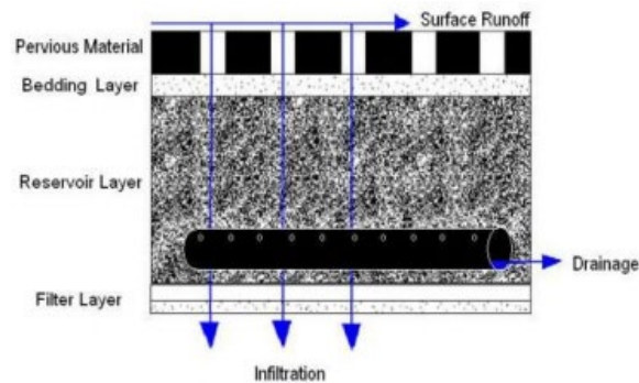
Figure 4: Typical Permeable Pavement Section
