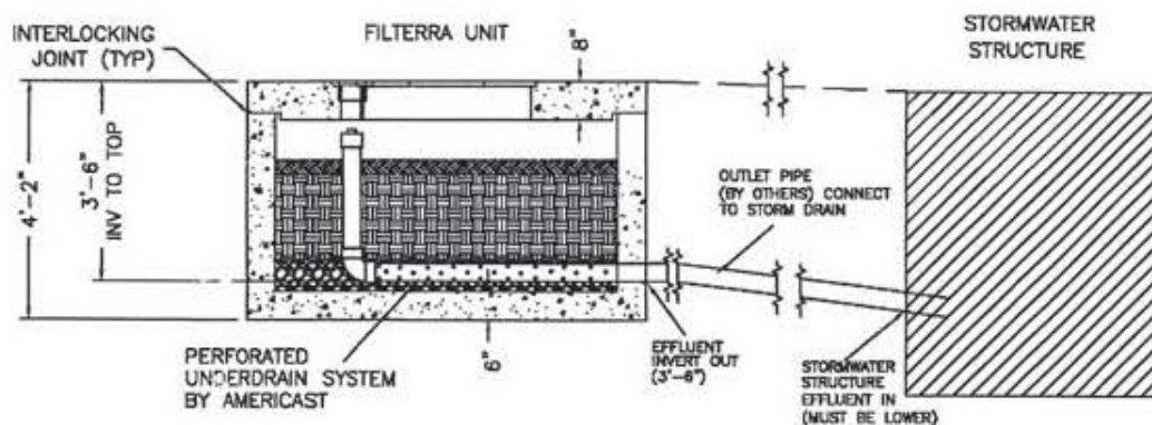
Figure 5: Typical Filterra Section
