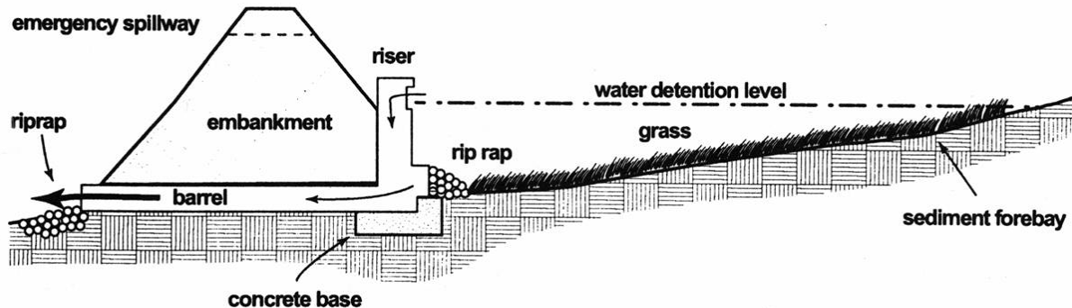
Figure 2: Typical Detention Basin Section
